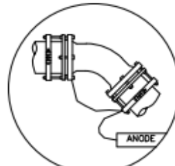
BENDS AND REDUCERS ARE TO BE PROTECTED WITH ONE (1) 7.7kg ANODE WITH JUMPER CABLE OR TWO (2) 2.7 kg ANODES CONNECTED INDIVIDUALLY. AN M.J. FITTING WITH RESTRAINTS REQUIRES ONE (1) 7.7 kg ANODE.
