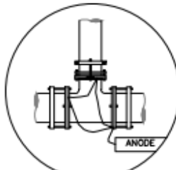
7.7 kg ANODE WITH JUMPER CONNECTIONS TO EACH OF THE THREE (3) RESTRAINTS ON THE PVC TEE OR CONNECTED DIRECTLY TO THE M.J. TEE. THE SAME APPLICATION APPLIES TO THE FOUR (4) RESTRAINTS ON A CROSS.
