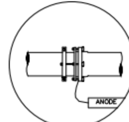
2.7 kg ANODE PER RESTRAINT OR ONE (1) 7.7 kg ANODE FOR THREE (3) RESTRAINTS IF WITHIN 3.0 m.
