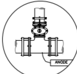
7.7 kg ANODE FOR EACH ANCHOR TEE AND VALVE WITH RESTRAINT ASSEMBLY
