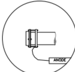
7.7 kg ANODE FOR A RESTRAINT ON A CAP OR A PLUG AT A DEAD END
